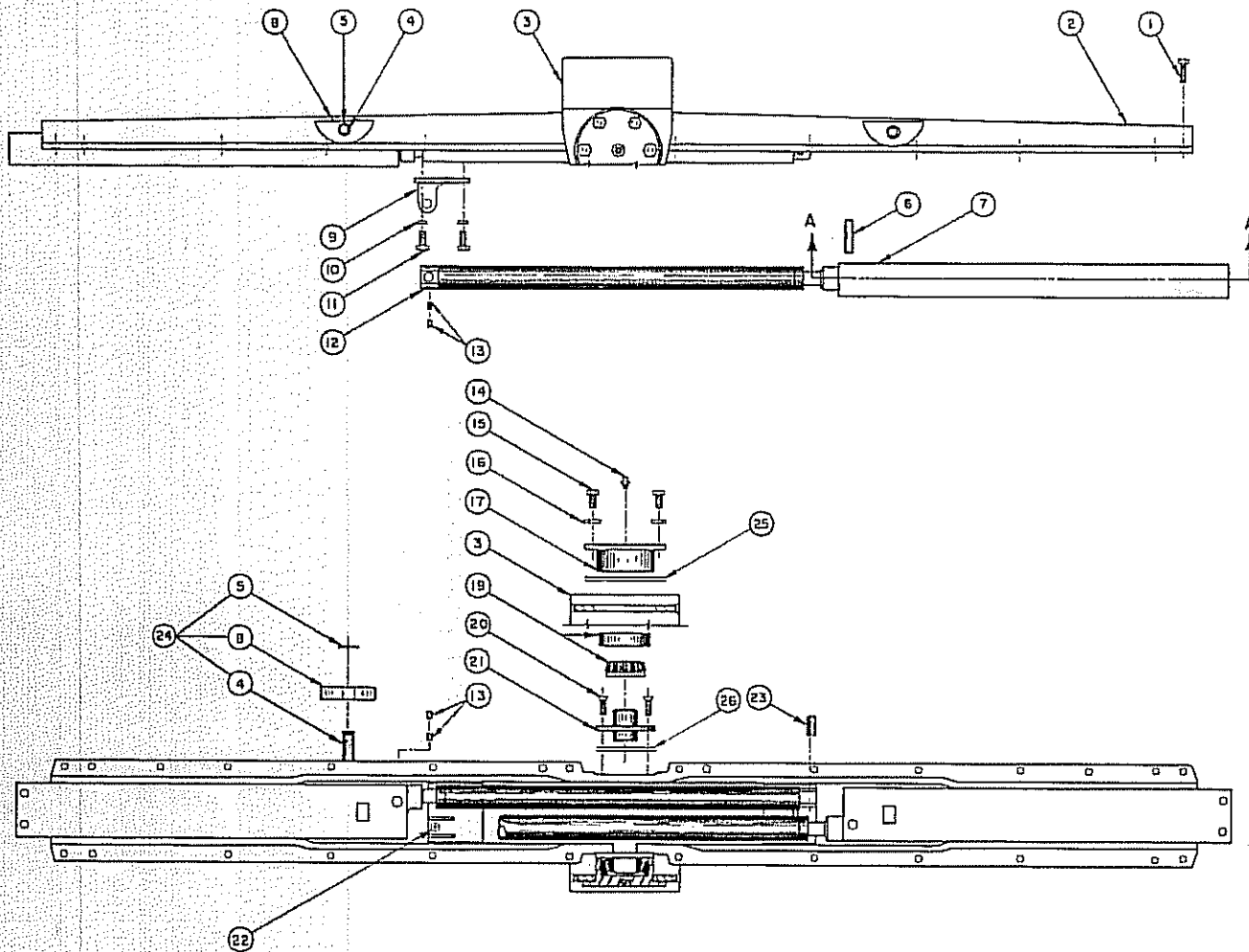
MAIN BEAM REAR HALF
