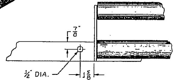
HOLE LOCATION FOR PAVERS PRIOR TO H-9084-B-D.
