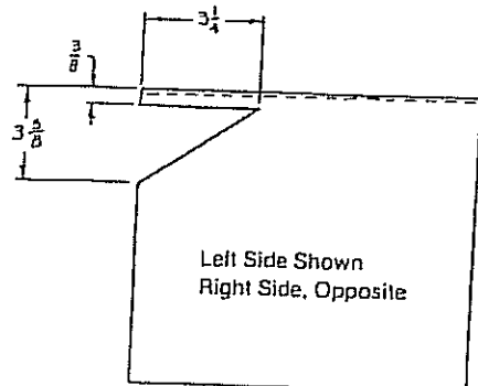
24" J.M.E.P. Screed Cover Cutout
